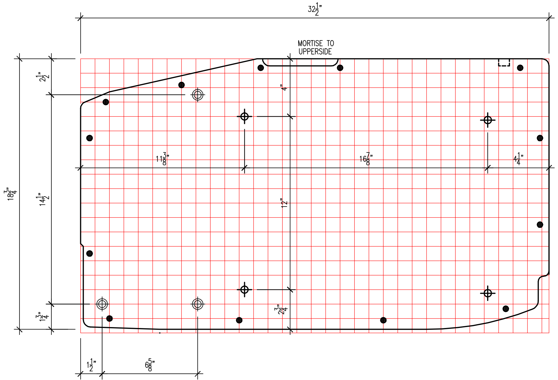
FLOORBOARD-REAR-L.H.
